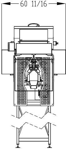
INFEED ELEVATION
