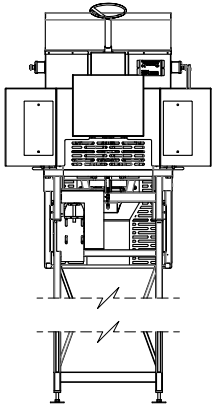
REAR ELEVATION
